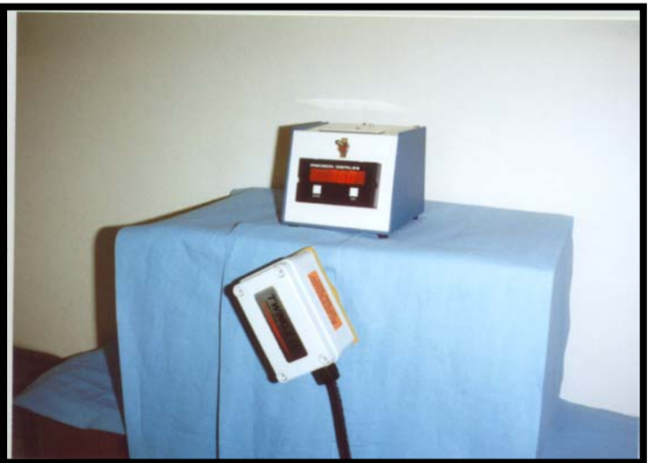
HOWDEEP display with signal brick tilted 60 degrees, indicating 76.0 feet digging depth.
