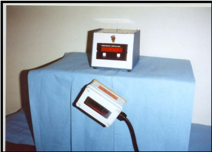
HOWDEEP display with signal brick tilted 45 degrees and indicating 44.9 feet digging depth.
