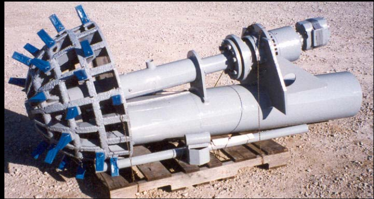
Top: K6-10 cutterhead Right: New K3-12 cutterhead ready for paint. Below: K6-14 cutterhead assembly, ready for shipping.
