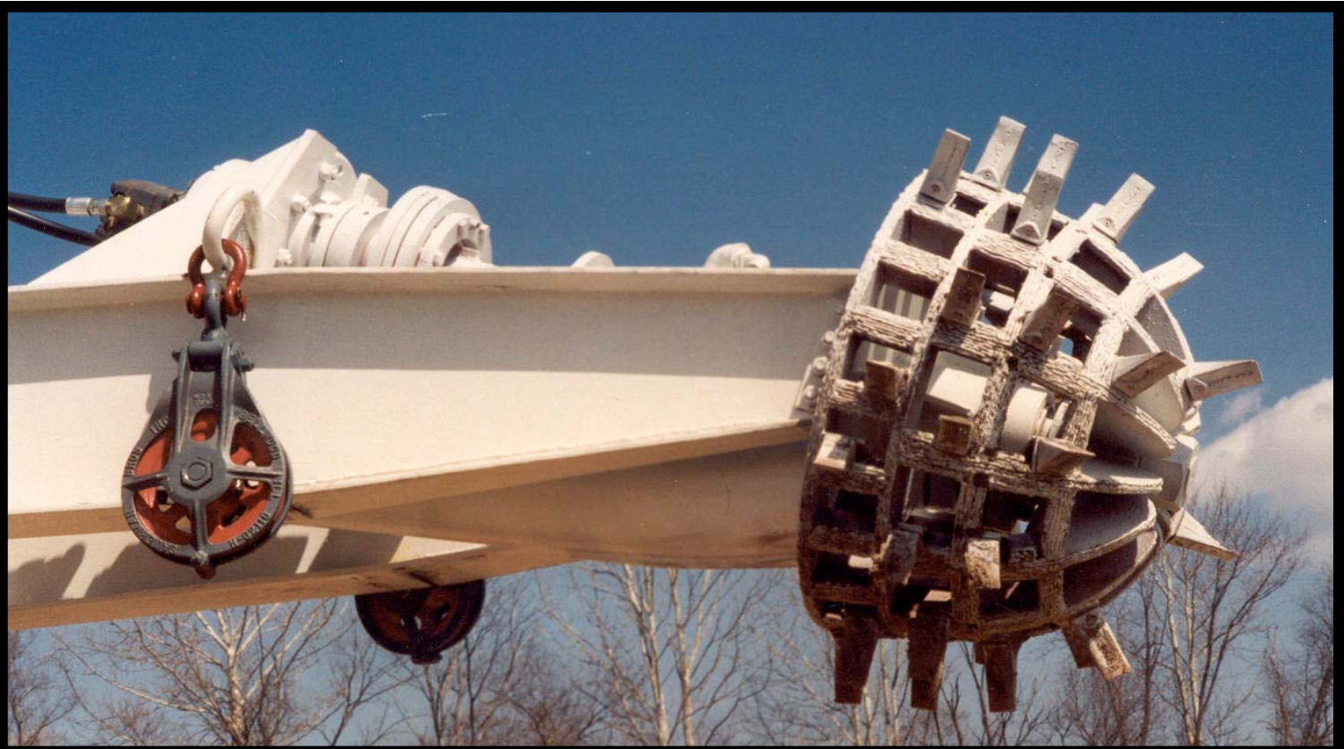
Top: K6-10 cutterhead Right: New K3-12 cutterhead ready for paint. Below: K6-14 cutterhead assembly, ready for shipping.
