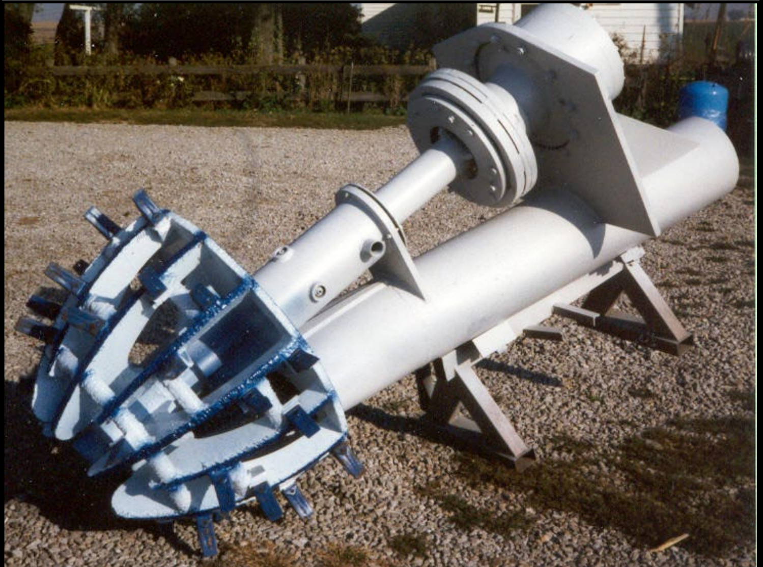
K252 Magnum cutterhead assembly with sand & gravel basket
