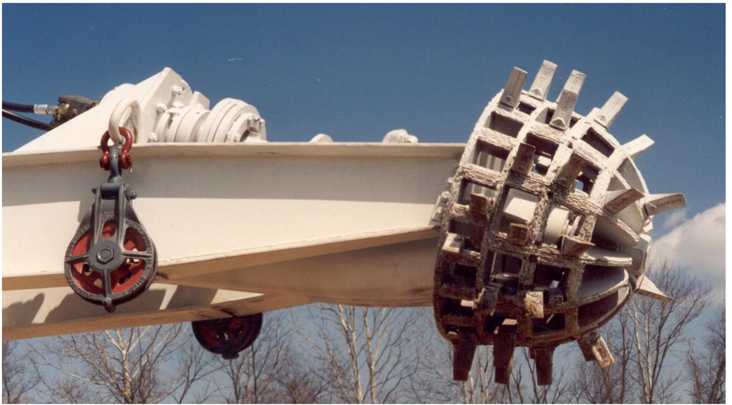
Top: K252-10 cutterhead
