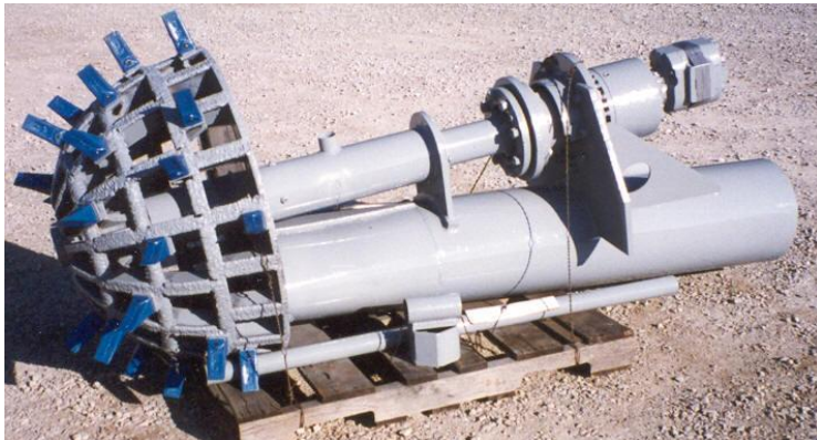
Below: K252-14 cutterhead assembly ready for shipping.
